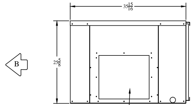
(1) 12"x12" Blower
