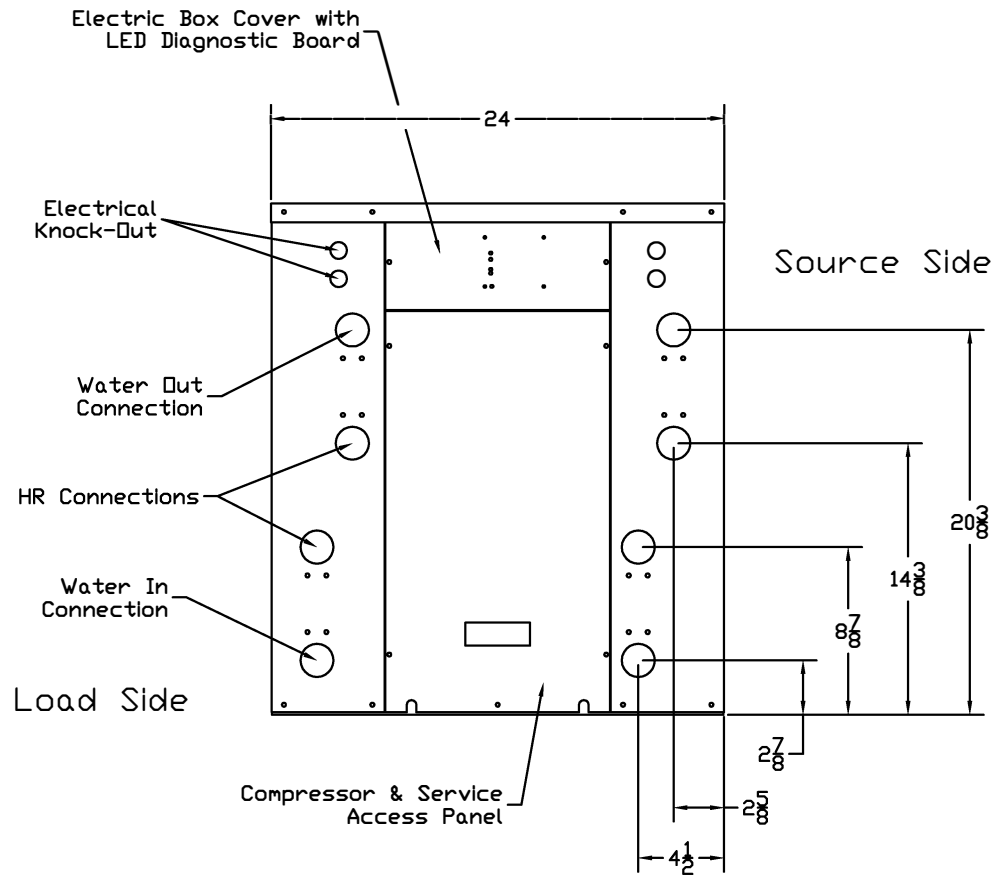
Front Elevation
